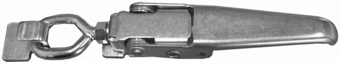
1.UES052053 Weld On Over centre Fastener ZP. Overall Length 220 -230mm. Base Plate 80mm x 30mm x 3mm.
