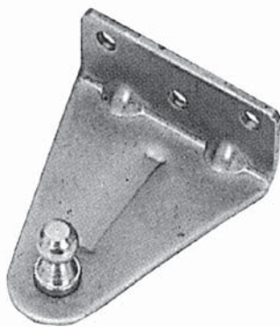
5.91003 Mounting bracket stainless steel. 54 x 66 x 43mm.
