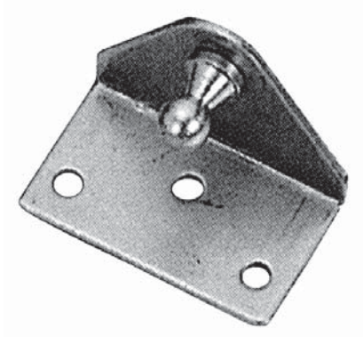
5.91008 Mounting bracket stainless steel. 51 x 19 x 34mm.
